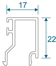
VL64 - Glazing Bead
