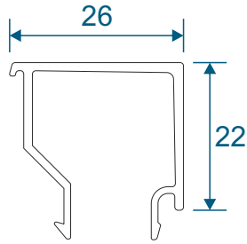
VL64 - Glazing Bead
