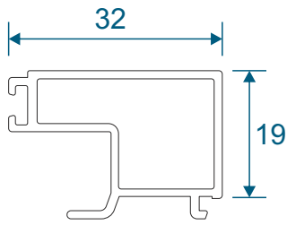
IMP613 - Glazing Bead
